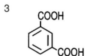
Isophthalic acid
